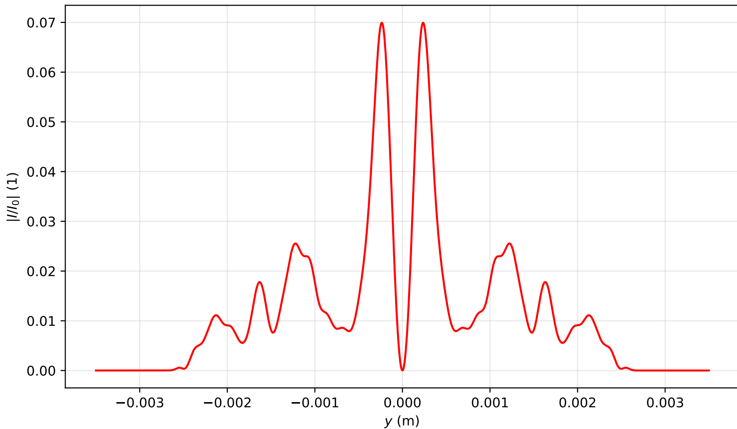
Intensity profile I(x=0, y, z=3.025)/I_0 , \text{Pin}=8.0\text{Pcr} , artificial time
